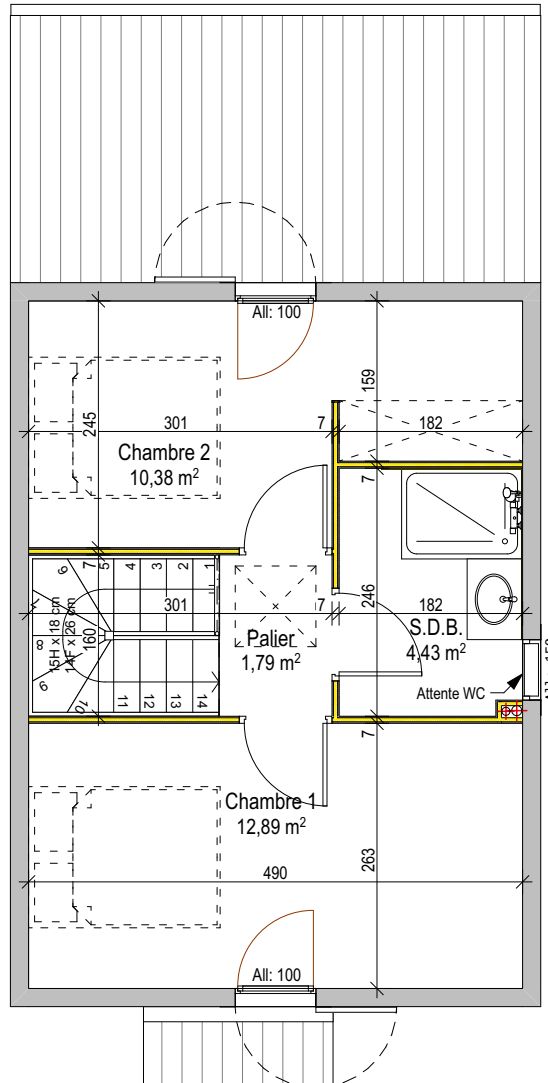
Plan R+1
