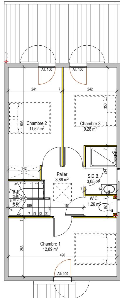
Plan R+1
