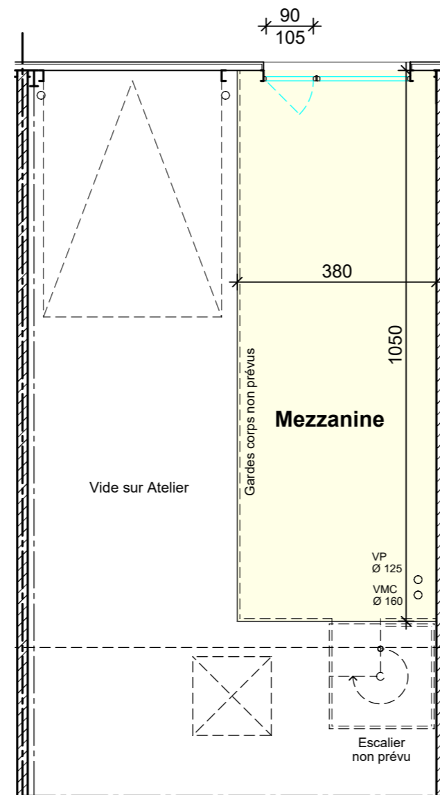
PLAN MEZZANINE
