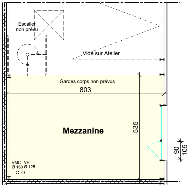
PLAN MEZZANINE
